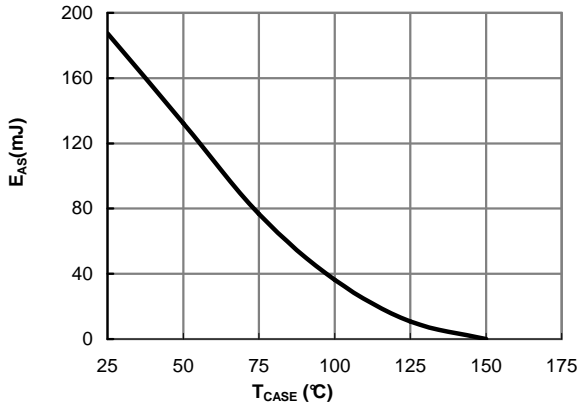
Figure 12: Avalanche energy
