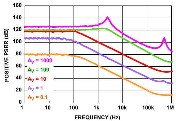
FIGURE 20. POSITIVE PSRR V_{EE} & V_{CC} ( R_F = 121k )
