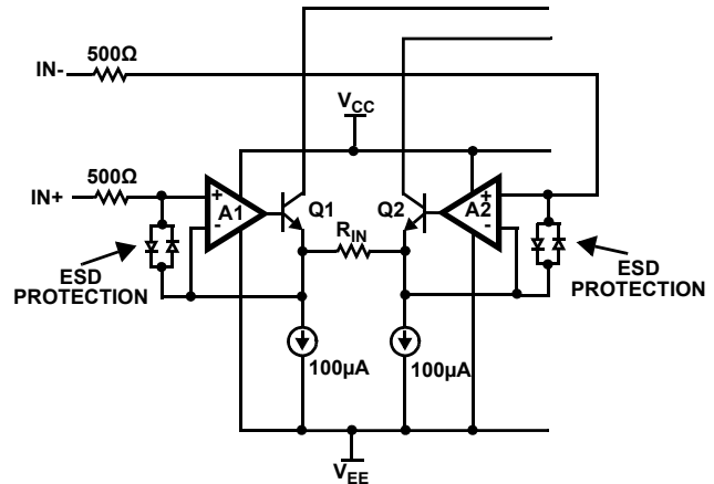
FIGURE 31. INPUT STAGE ESD PROTECTION DIODES
