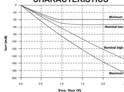
FIGURE B – FULL DRIVE PULL-UP CHARACTERISTICS
