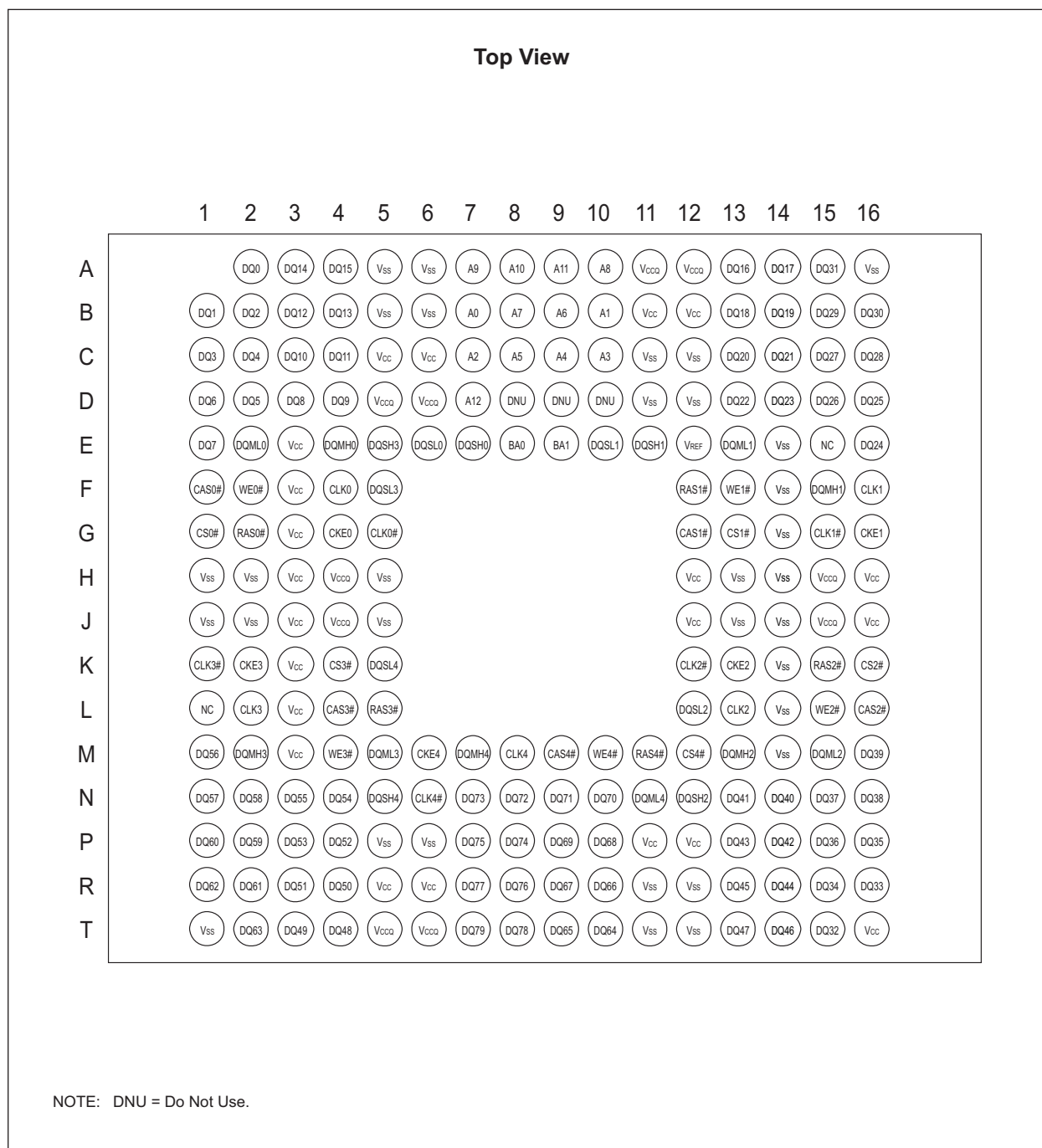
FIGURE 1 – PIN CONFIGURATION
