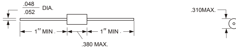
FIG.3 PACKAGE STYLE
