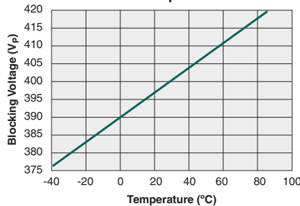
Form-A Typical Blocking Voltage vs. Temperature
