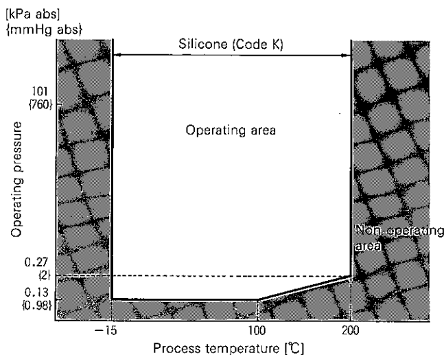
Fig. 2 Relation between process temperature and operating pressure
