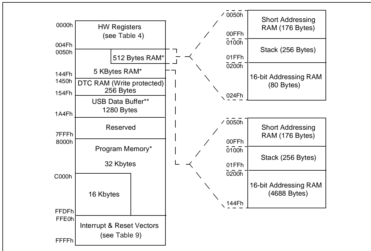
Figure 9. Memory Map
