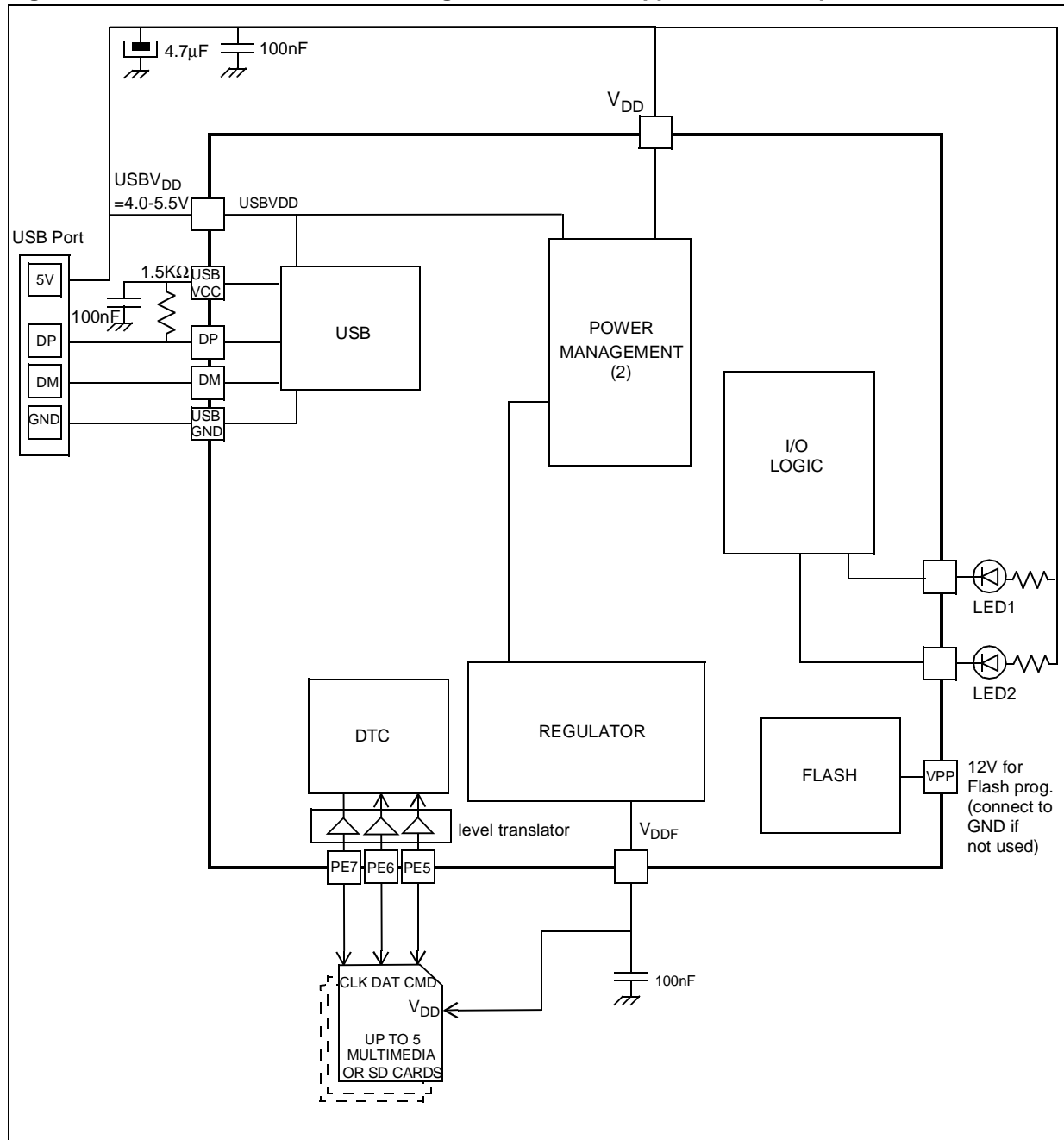
Figure 5. Multimedia Card Or Secure Digital Card Writer Application Example
