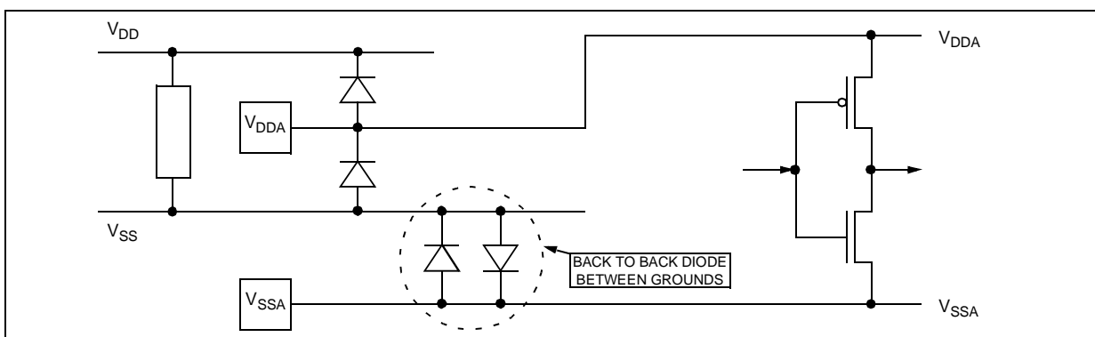
Figure 84. Multisupply Configuration
