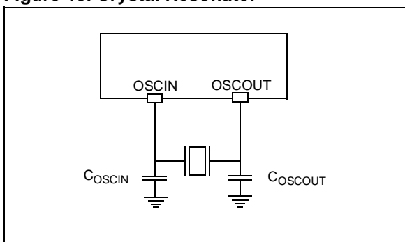
Figure 15. Crystal Resonator
