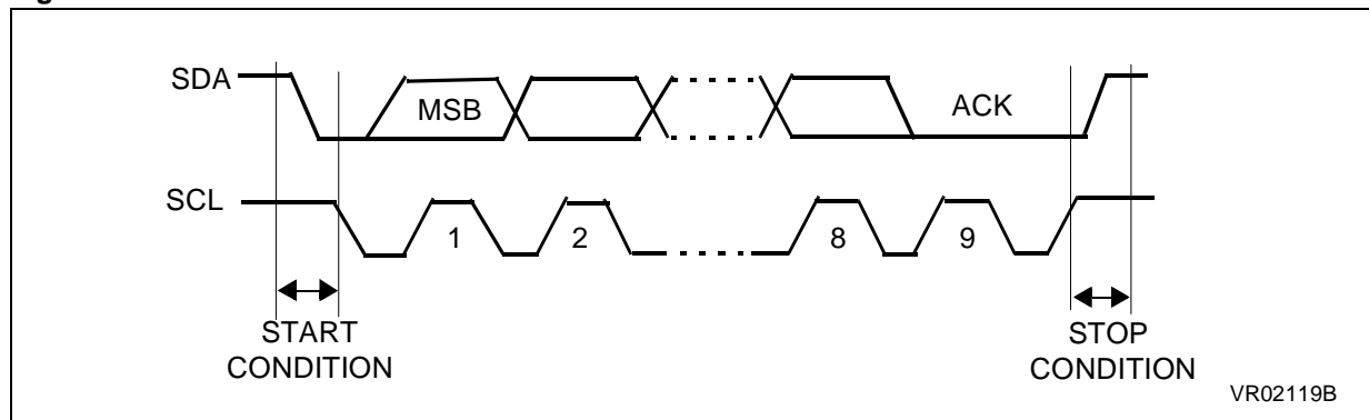
Figure 64. I 2 C BUS Protocol
