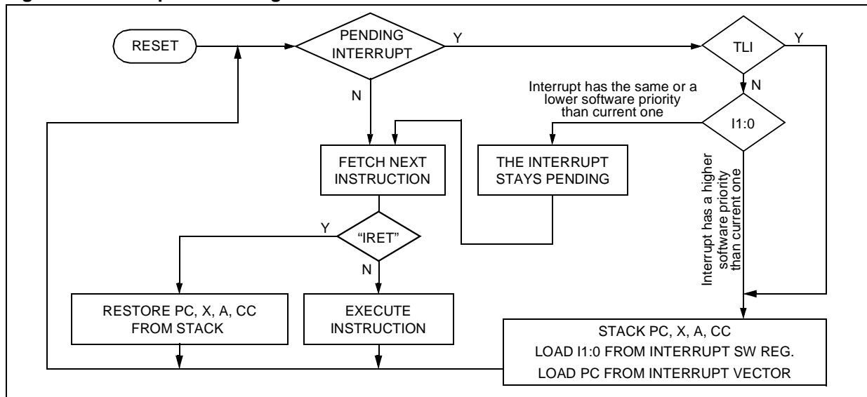
Figure 27. Interrupt Processing Flowchart
