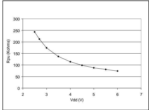
Figure 88. Typical R_{PU} vs. V_{DD} with V_{IN}=V_{SS}
