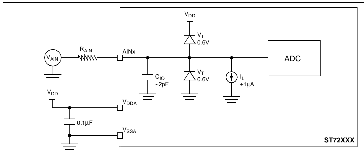
Figure 102. Typical Application with ADC
