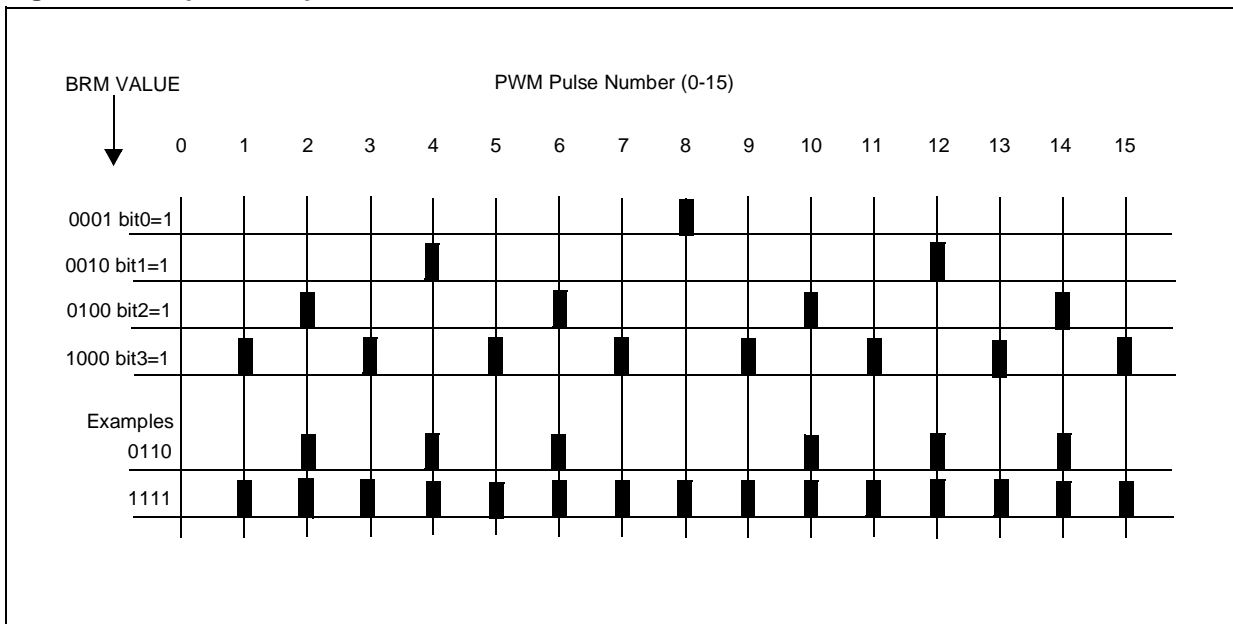
Figure 55. Graphical Representation of 4-Bit BRM Added Pulse Positions
