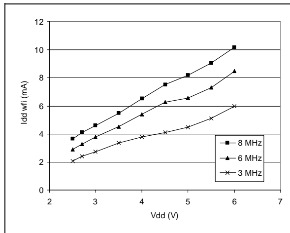
Figure 74. Typical I_{DD} in WAIT vs. f_{CPU}
