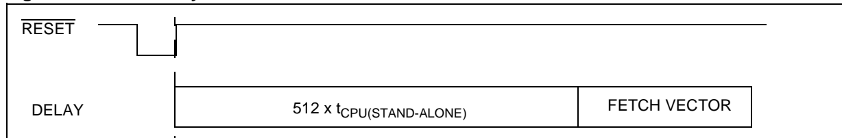
Figure 18. Reset Delay in Stand-alone Mode
