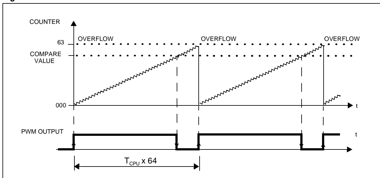
Figure 50. PWM Generation
