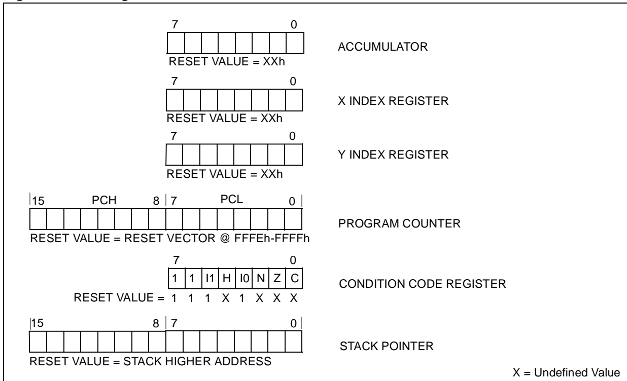
Figure 12. CPU Registers
