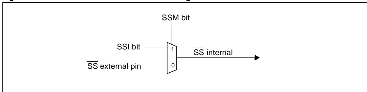
Figure 60. Hardware/Software Slave Select Management
