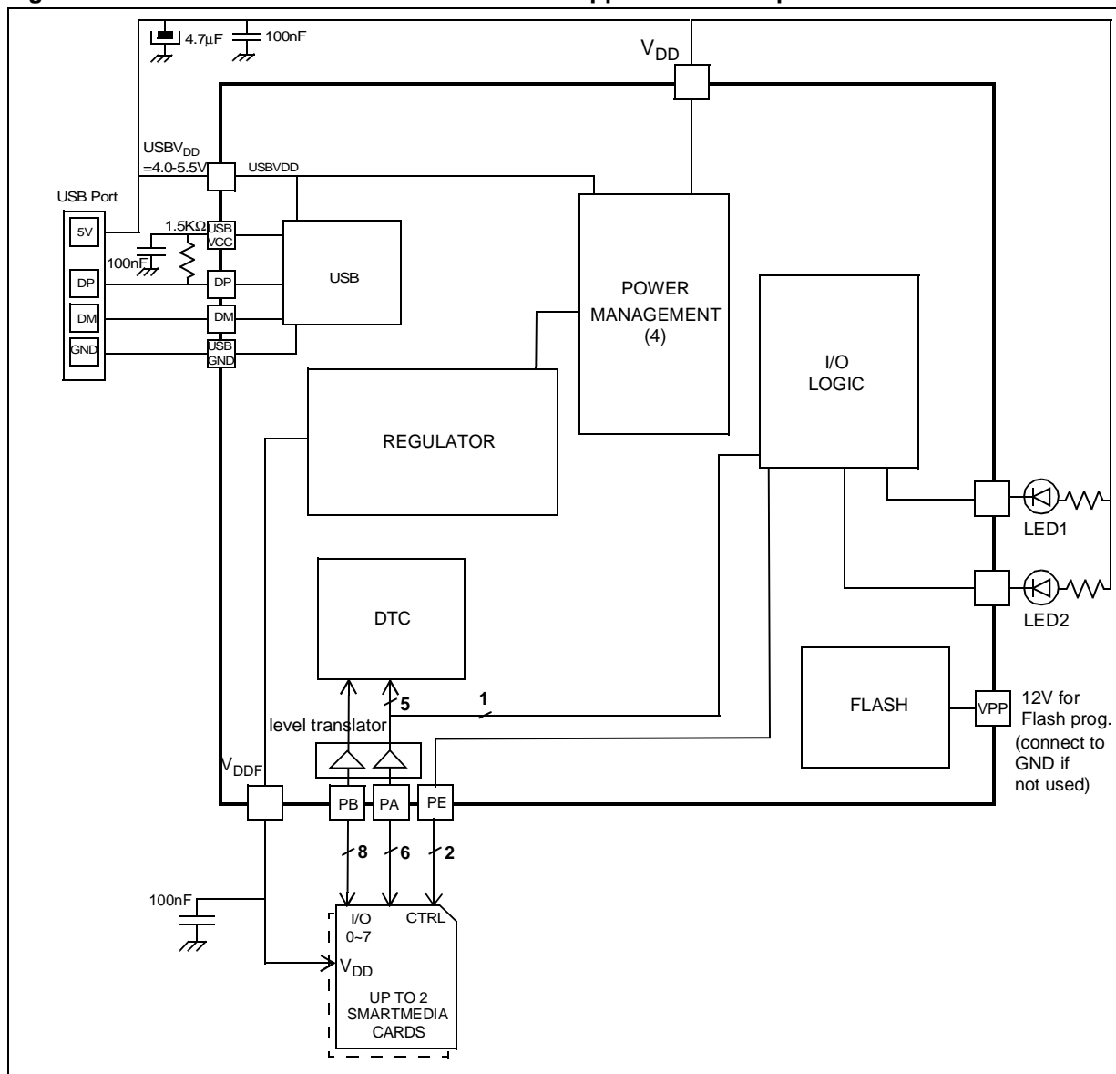
Figure 6. Smartmedia Card Writer Or Flash Drive Application Example
