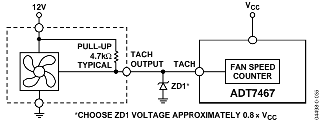
Figure 43. Fan with TACH Pull-Up to Voltage > 5 V. (for example, 12 V) Clamped with Zener Diode
