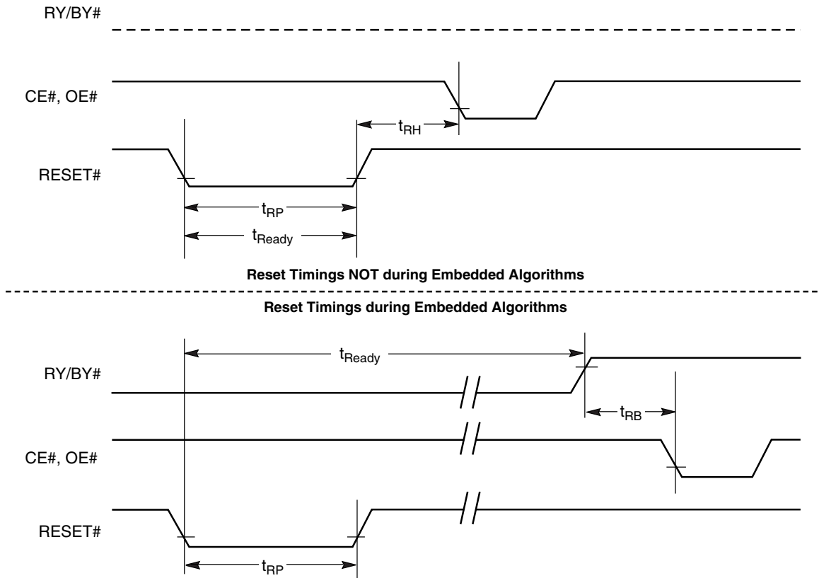
Figure 15. Reset Timings
