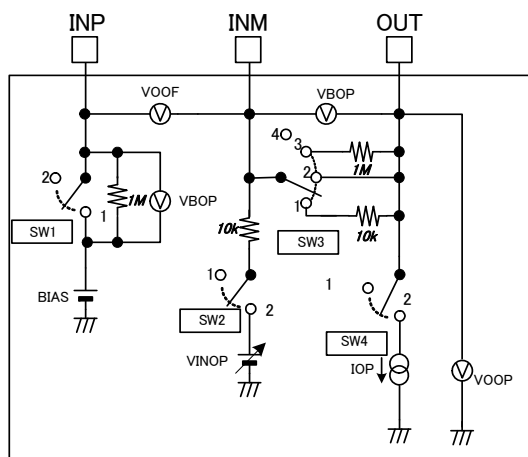
Figure5 TEST CIRCUIT
