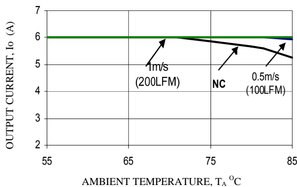
V_o = 3.3V
