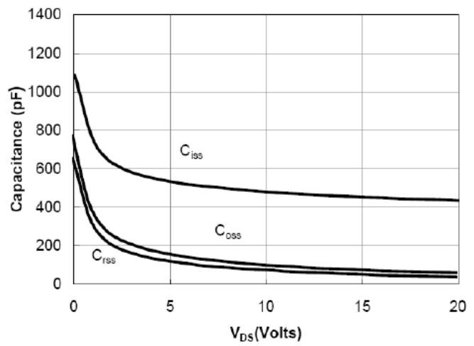
Figure 8: Capacitance Characteristics
