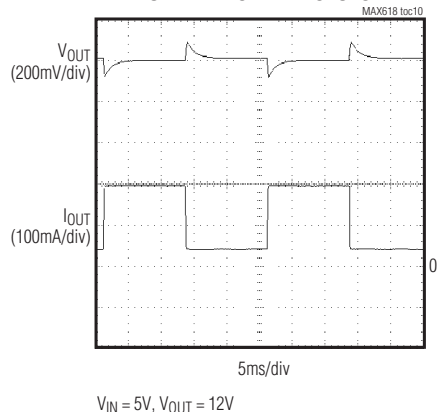
LOAD-TRANSIENT RESPONSE
