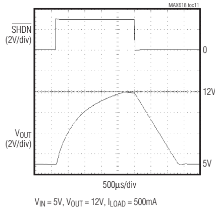
SHUTDOWN RESPONSE
