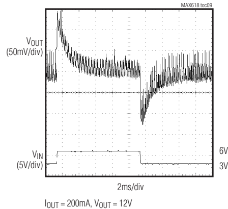
LINE-TRANSIENT RESPONSE
