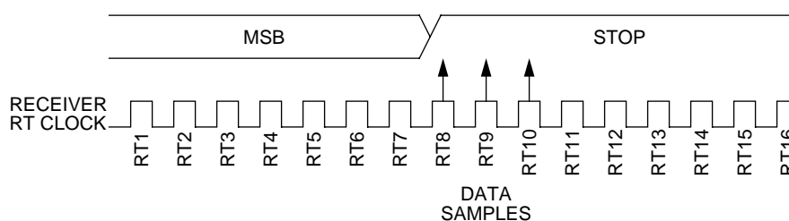
Figure 15-7. Slow Data
