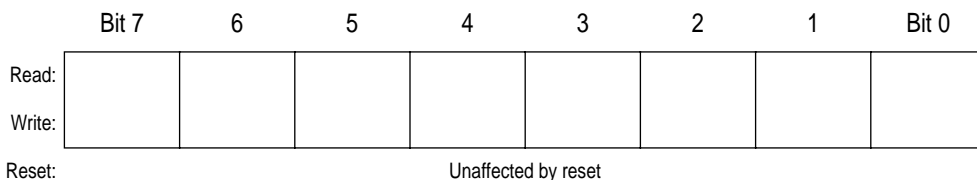
Figure 7-2. Accumulator (A)
