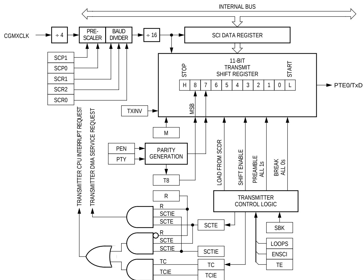
Figure 15-4. SCI Transmitter
