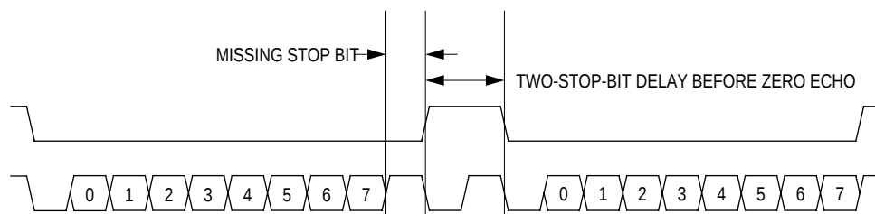
Figure 10-5. Break Transaction
