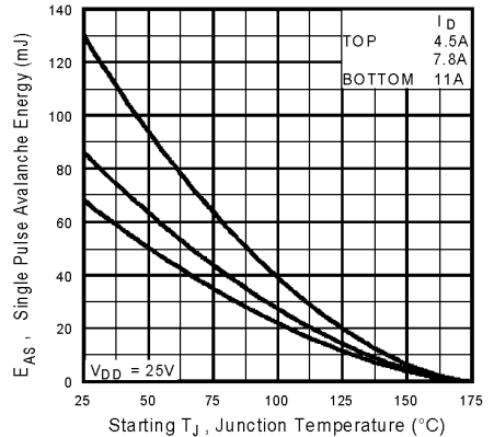
Fig 12c. Maximum Avalanche Energy Vs. Drain Current
