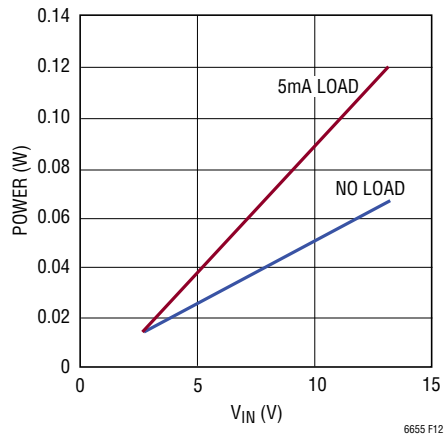
Figure 12. LTC6655-2.5 Power Consumption
