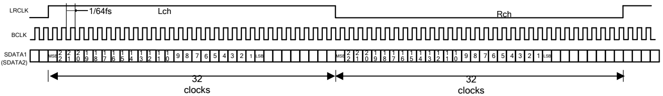
Fig.23 Left-Justified Data Format 64fs, 24 bit Data
