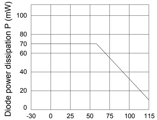
Diode Power Dissipation vs. Ambient Temperature
