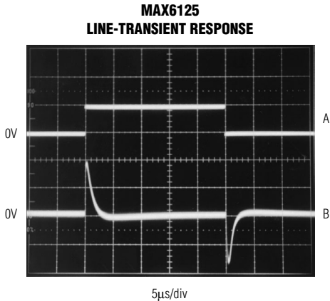
A = INPUT VOLTAGE, 100mV/div, V_{IN} = 3V \pm 50mV B = OUTPUT VOLTAGE, 20mV/div
