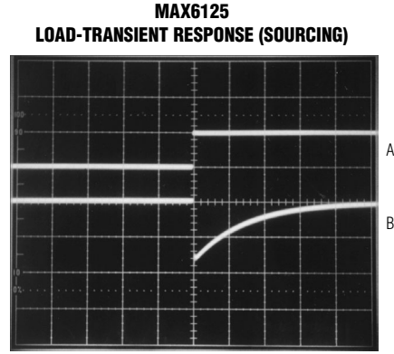
A = OUTPUT CURRENT, 1mA/div, I_{OUT} = 0mA to 1mA B = OUTPUT VOLTAGE, 50mV/div
