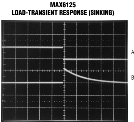
A = OUTPUT CURRENT, 1mA/div, I_{OUT} = 0mA to -1mA B = OUTPUT VOLTAGE, 200mV/div
