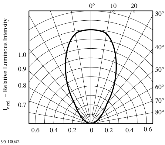
Figure 19 Rel. Luminous Intensity vs. Angular Displacement
