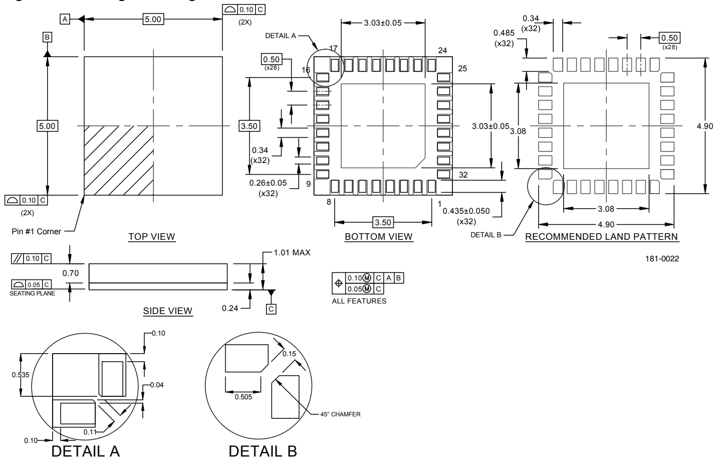
Figure 23. Package Drawing
