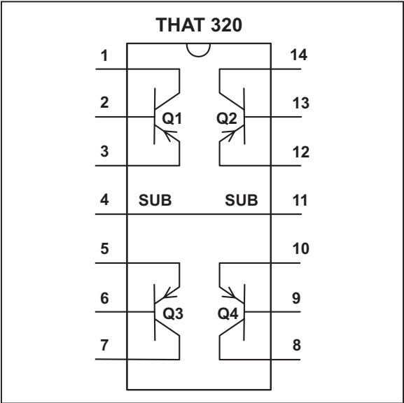
Fig 2. 320 Pinout
