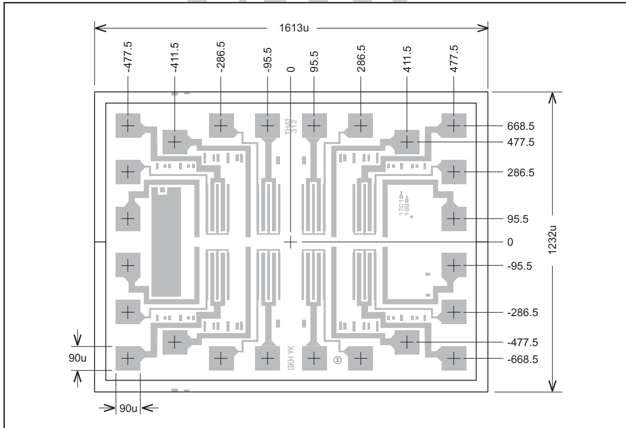
Figure 7. Die dimensions
