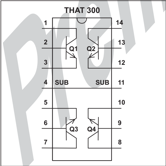
Fig 1. 300 Pinout
