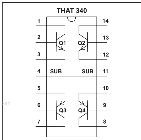
Fig 3. 340 Pinout
