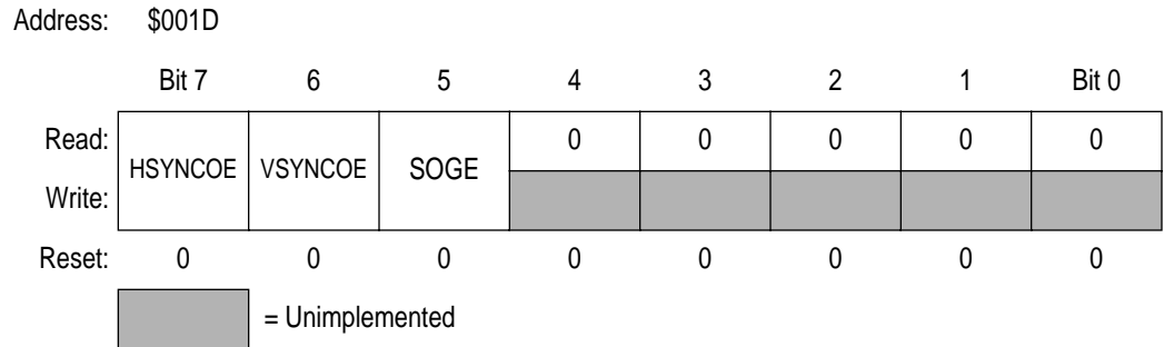
Figure 15-19. Configuration Register 0 (CONFIG0)
