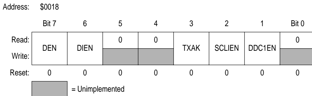
Figure 13-3. DDC Control Register (DCR)
