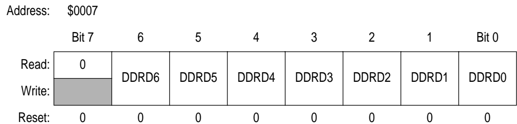
Figure 15-13. Data Direction Register D (DDRD)
