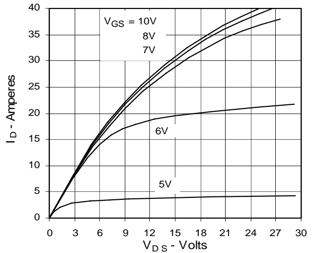
Fig. 2. Output Characteristics @ 125°C
