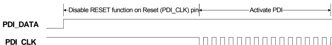
Figure 22-3. Sequence for enabling the PDI.
