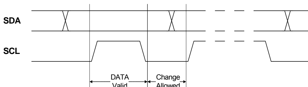
Figure 16-4. Data Validity
