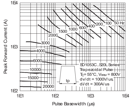
Fig. 31 - Frequency Characteristics
