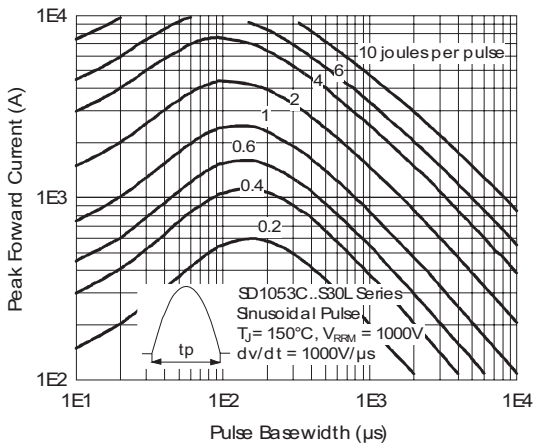
Fig. 34 - Maximum Total Energy Loss Per Pulse Characteristics
