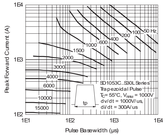
Fig. 37 - Frequency Characteristics
