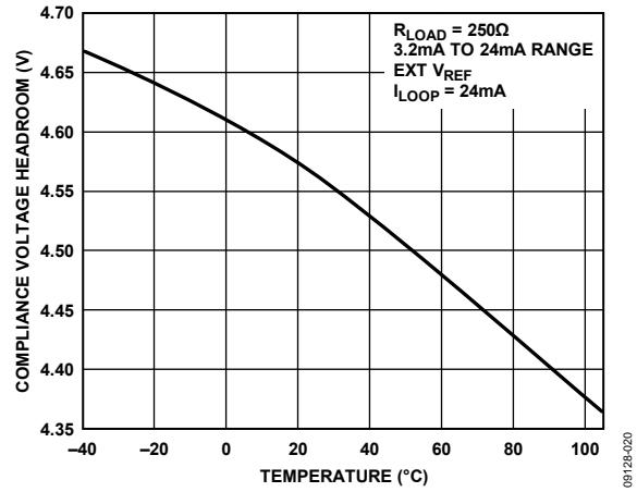
Figure 20. Compliance Voltage Headroom vs. Temperature
