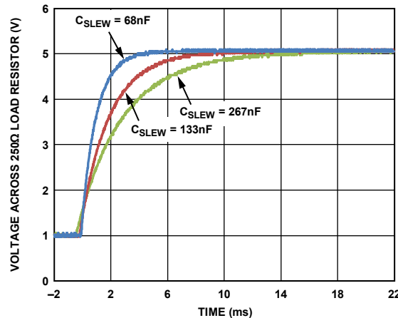
Figure 44. 4 mA to 20 mA Step with Slew Rate Control
