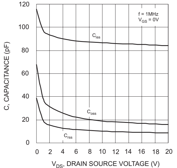
Fig. 12 Capacitance Variation
