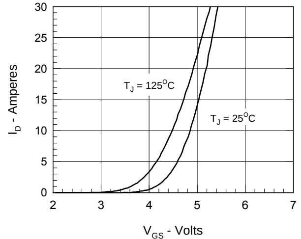
Figure 4. Admittance Curves
