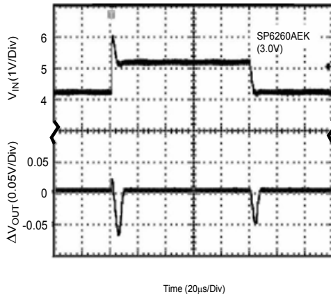
SP6260EAK (3.0V) Line Transient (Conditions: I_{OUT}=30\text{mA} , C_{IN}=1\mu\text{F} , C_{OUT}=1\mu\text{F} )
