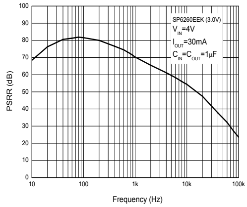
PSRR vs. Frequency SP6260EEK (3.0V)
