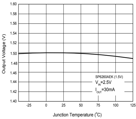
SP6260AEK-L (1.5V) Output Voltage vs. Junction Temperature
