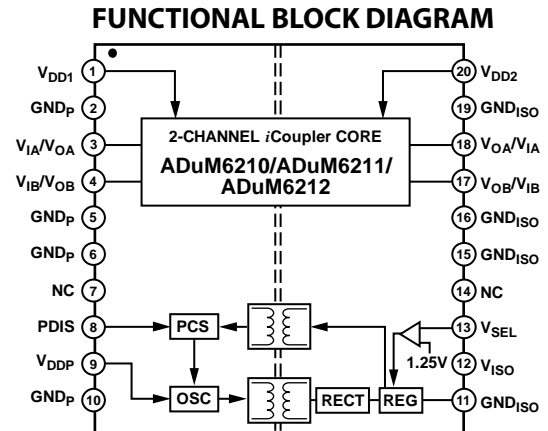
Figure 1. ADuM6210/ADuM6211/ADuM6212
