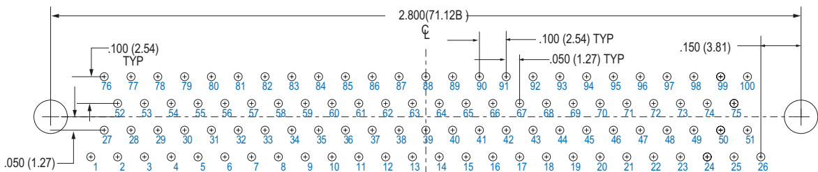
100 SOCKET MWDM-100SBS
