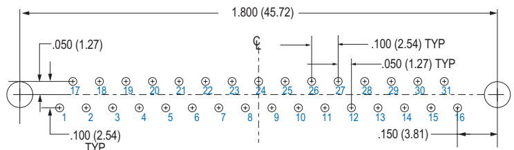
31 SOCKET MWDM-31SBS
