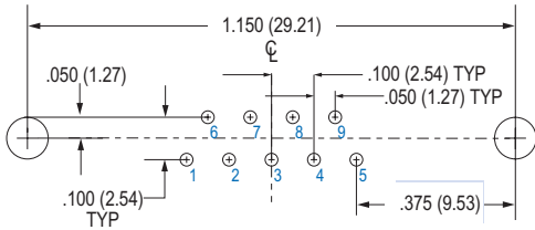
9 SOCKET MWDM-9SBS
