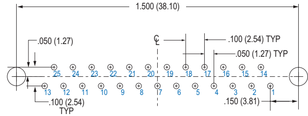
25 PIN MWDM-25PBS
