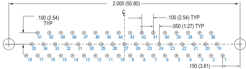
51 PIN MWDM-51PBS
