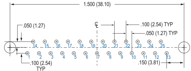
25 SOCKET MWDM-25SBS
