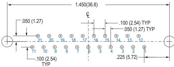
21 PIN MWDM-21PBS
