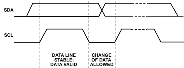
Figure 54. Valid Bit Transfer
