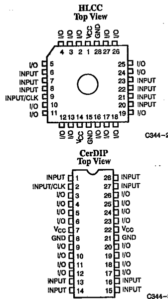
Pin Configurations
