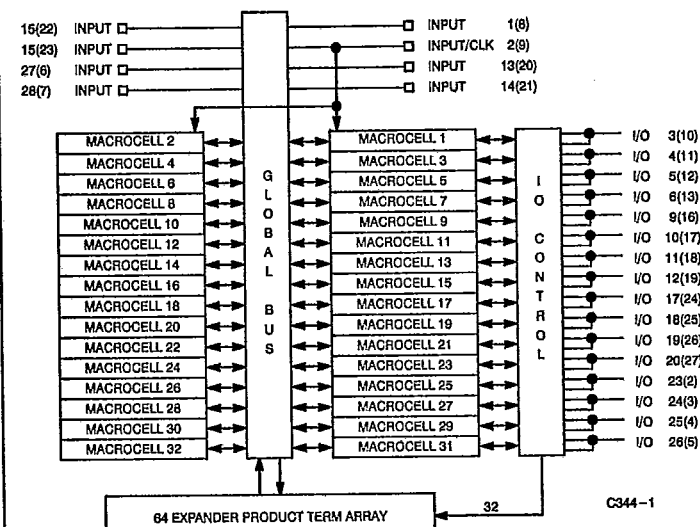
Logic Block Diagram [1]
