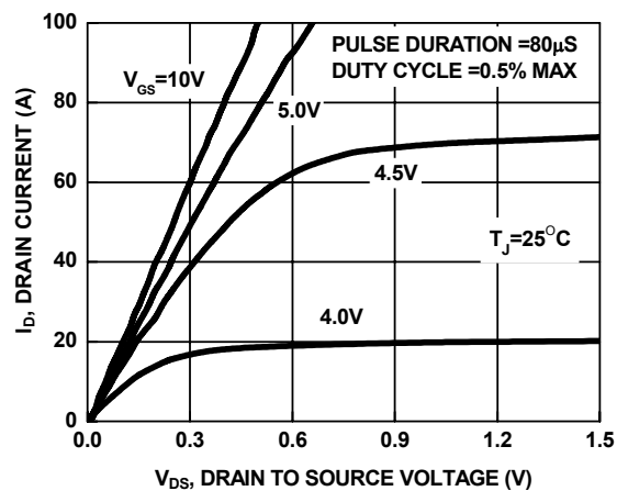
Figure 8. Saturation Characteristics
