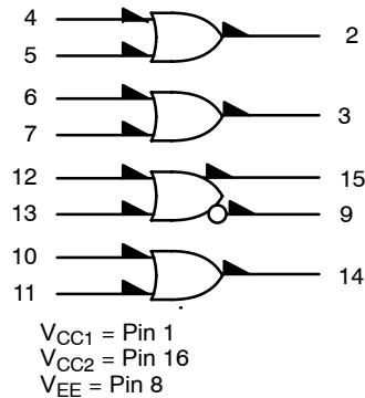
Figure 1. Logic Diagram
