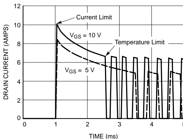
Figure 9. Short-circuit Response
