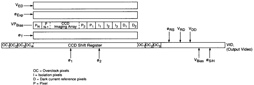
Figure 3. Simplified Schematic of the DE Series Linear Array
