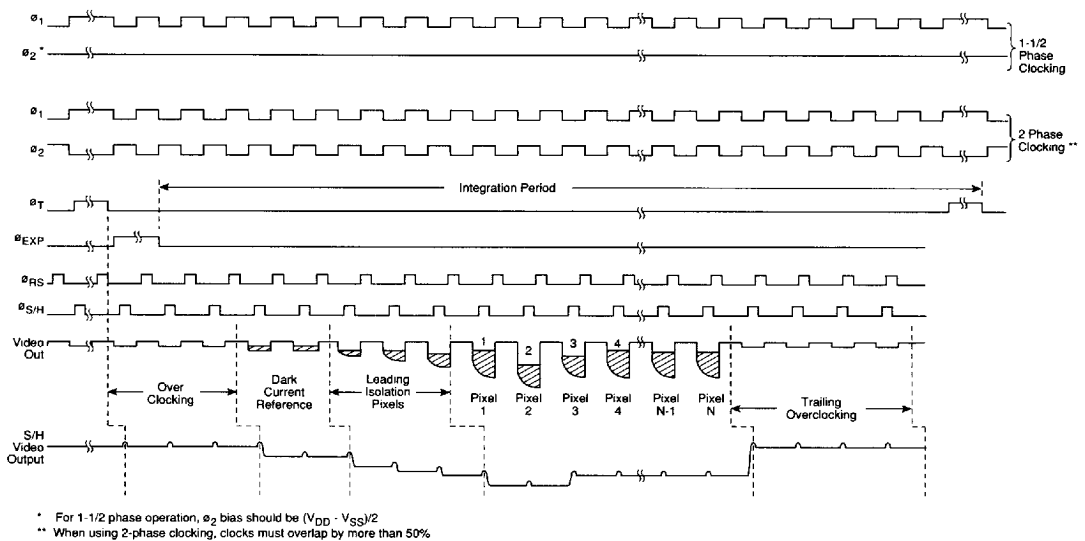
Figure 4. Timing Diagram
