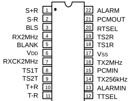
22 Lead PDIP (0.400")
