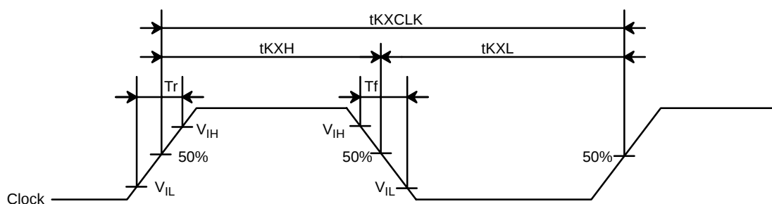
Figure 5. Clock Timing
