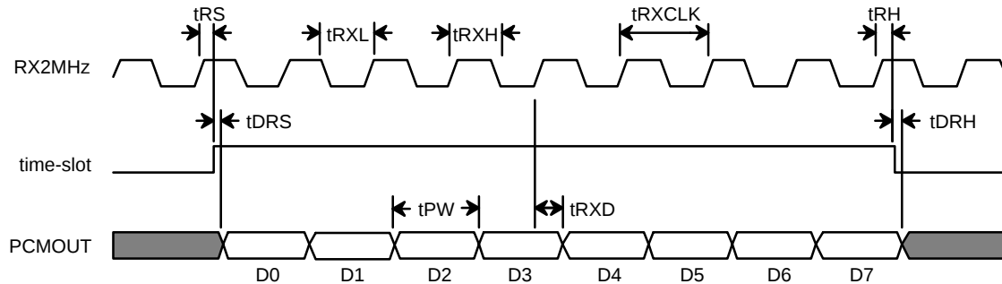
Figure 3. Receive Time-slot Timing
