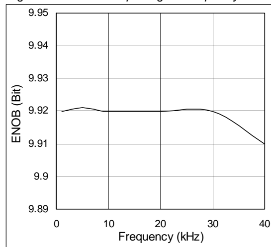
Figure 9. ENOB vs. Input Signal Frequency
