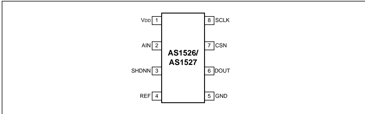
Figure 22. Pin Assignments (Top View)
