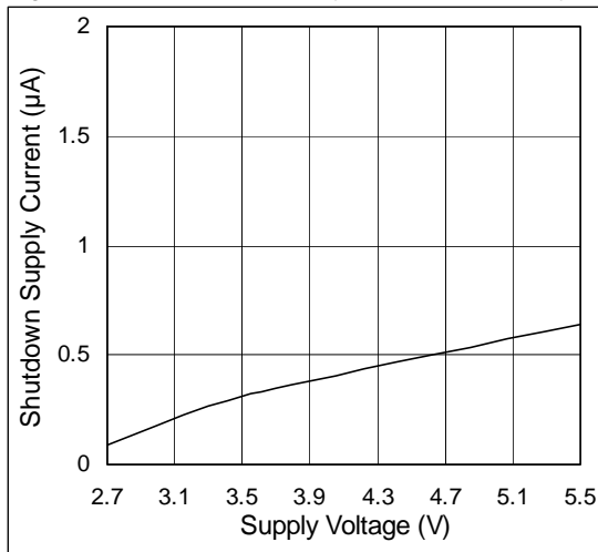
Figure 12. Shutdown Supply Current vs. Supply Voltage
