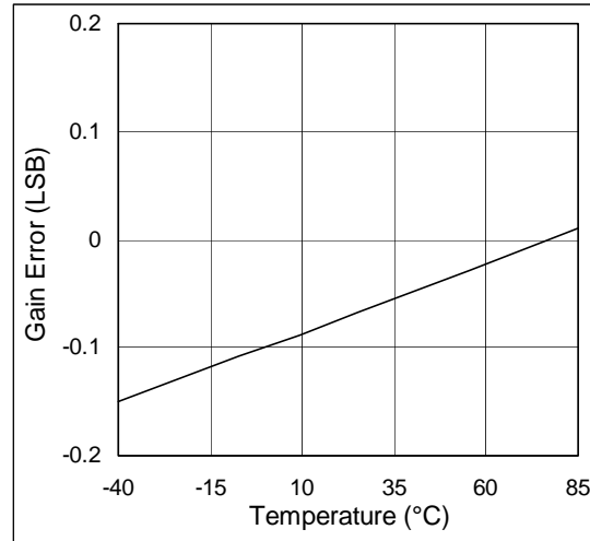
Figure 17. Gain Error vs. Temperature
