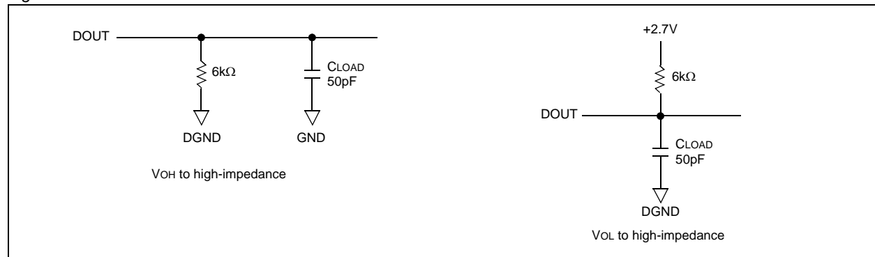
Figure 3. DOUT Disable-Time Load Circuits
