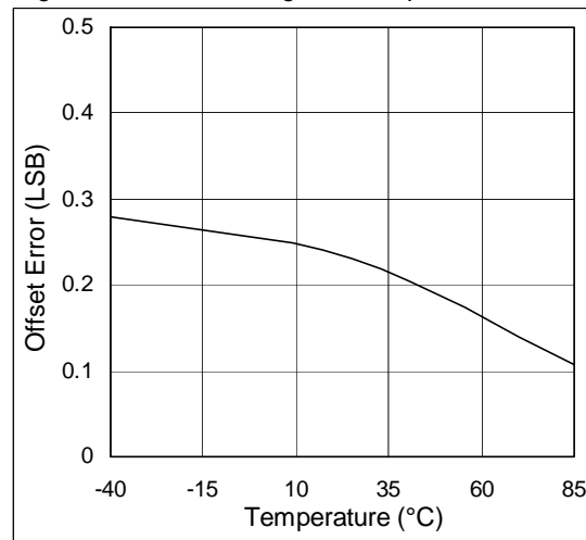
Figure 15. Offset Voltage vs. Temperature
