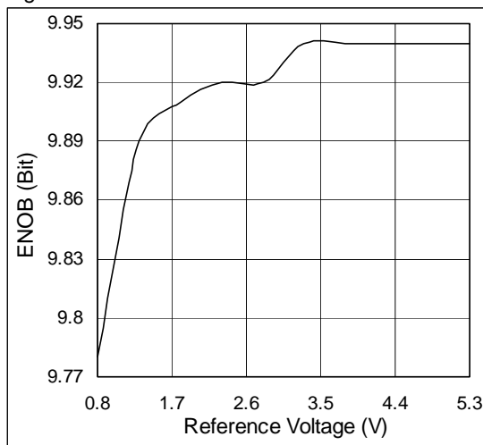
Figure 8. ENOB vs. V_{REF}
