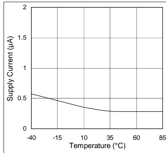
Figure 13. Shutdown Supply Current vs. Temperature
