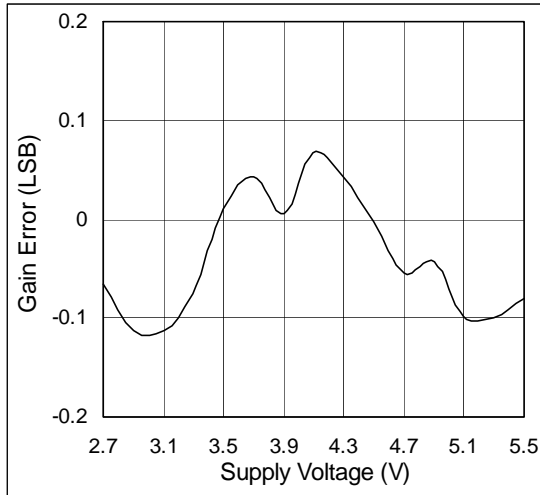
Figure 16. Gain Error vs. Supply Voltage
