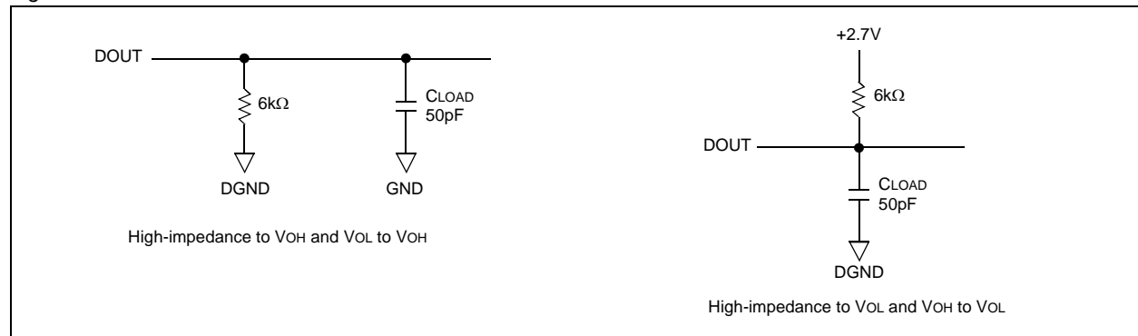
Figure 2. DOUT Enable-Time Load Circuits
