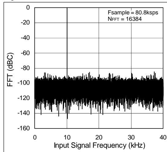
Figure 7. FFT @ 10kHz
