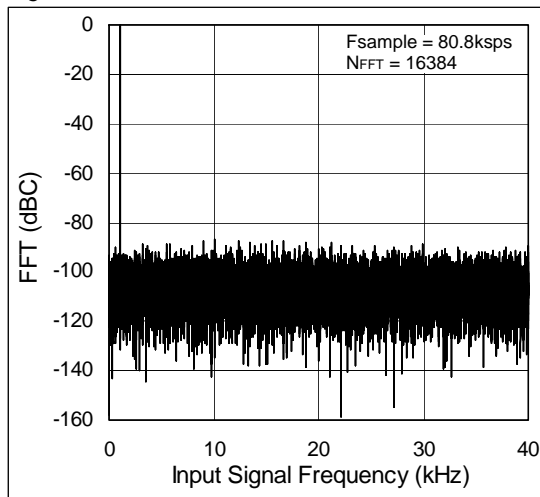
Figure 6. FFT @ 1kHz
