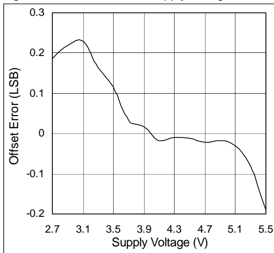
Figure 14. Offset Error vs. Supply Voltage
