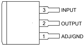
S Package (TO-263-3)
