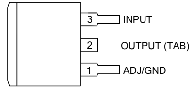
S2 Package (TO-263-2)
