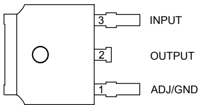
(TO-252-2 (3))
