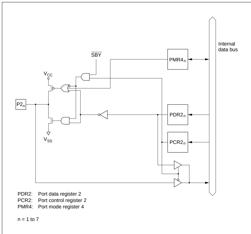
Figure C-2 (a) Port 2 Block Diagram (Pins P2 7 to P2 1 )
