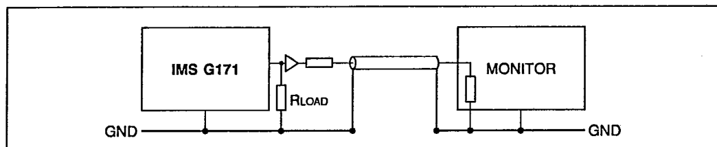
Figure 3.15 Buffered signal
