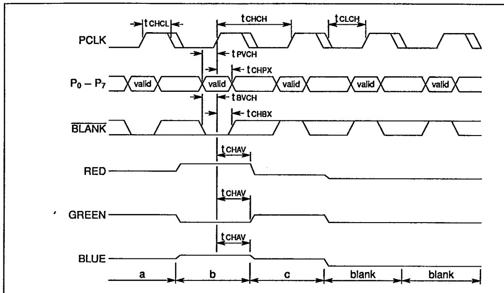
Figure 3.4 Video operation
