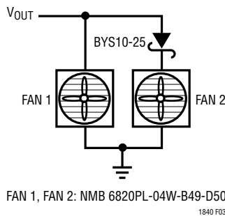
Figure 3. Series Diode to Avoid Beat Frequencies
