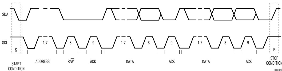
Typical 2-Wire Serial I 2 C or SMBus Transmission
