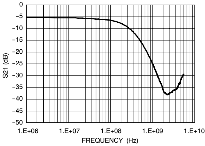
Figure 1. Typical Insertion Loss Characteristic
