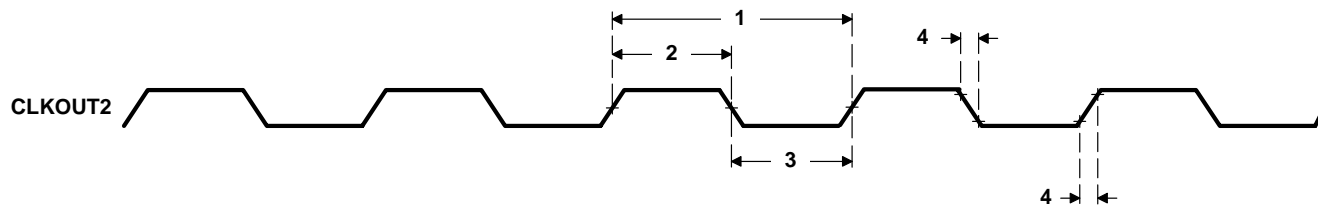
Figure 12. CLKOUT2 Timings
