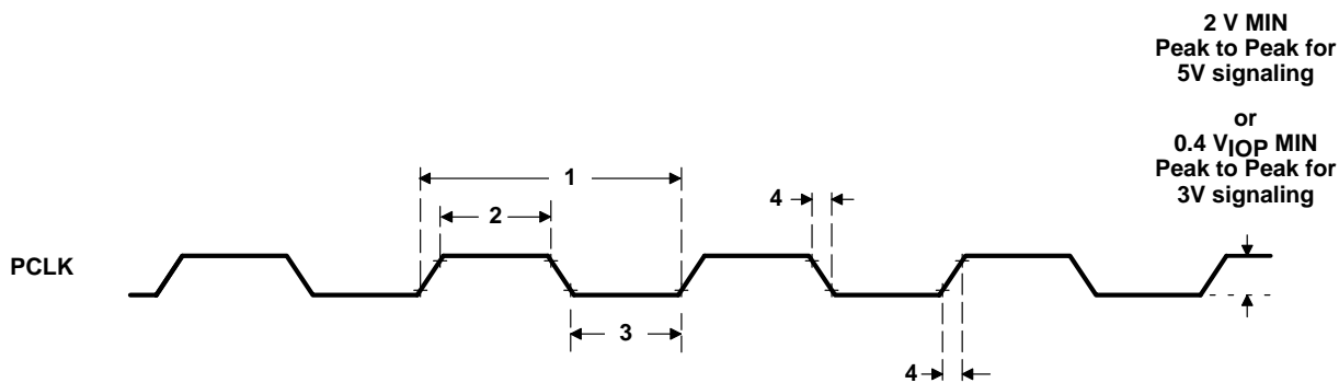
Figure 11. PCLK Timings
