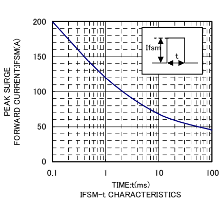
IFSM-t CHARACTERISTICS
