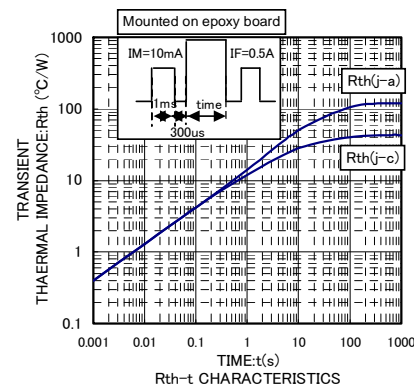
Rth-t CHARACTERISTICS
