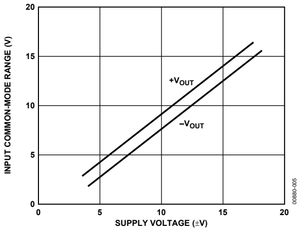
Figure 5. Input Common-Mode Range vs. Supply Voltage
