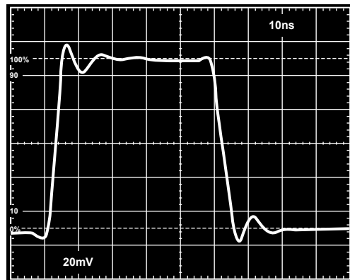
Figure 43. Small Signal Pulse Response of Inverting Amplified Using Current Feedback Compensation, C_{COMP} = 4 pF, R_F = 1 k \Omega , R1 = 1 k \Omega
