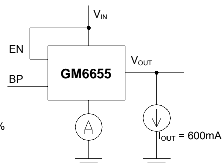
Fig 5. Load Regulation
