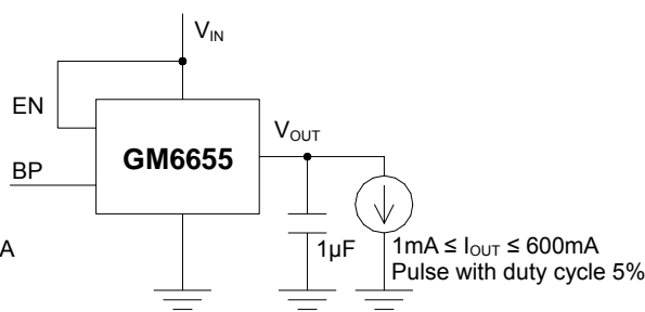
Fig 4. Load Regulation
